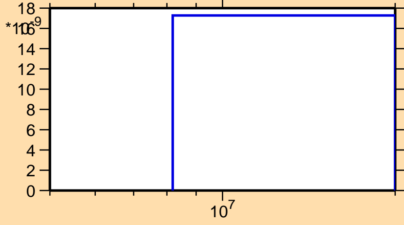
\sigma vs. E for ^{137}\text{Sm} (mt 45)
