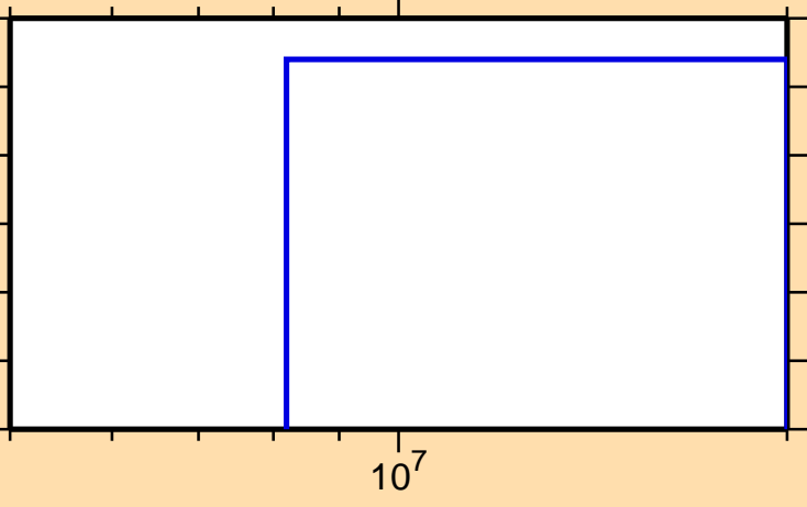
\sigma vs. E for ^{137}\text{Sm}(n,\text{pd})
