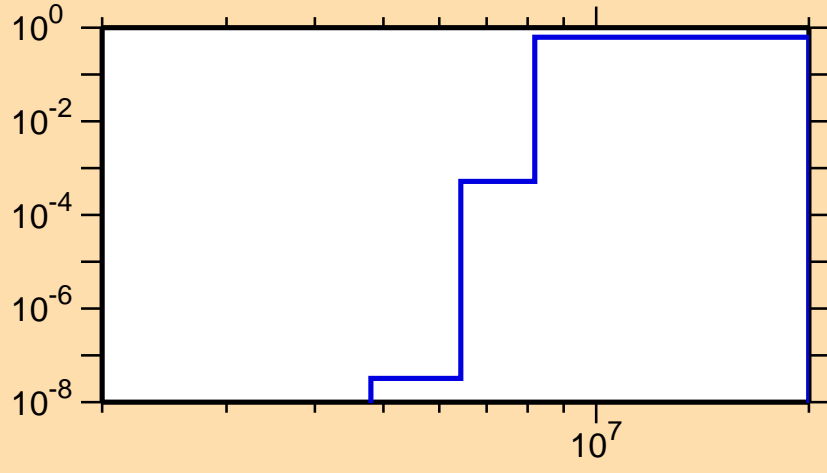
\sigma vs. E for ^{137}\text{Sm}(n,np)
