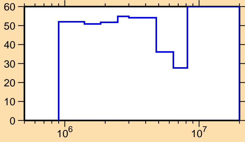
\Delta\sigma/\sigma vs. E for ^{137}\text{Sm}(n,ncont.)
