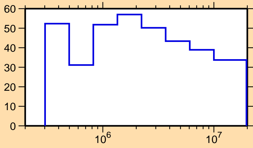
\Delta\sigma/\sigma vs. E for ^{138}\text{Sm}(n,n_1)
