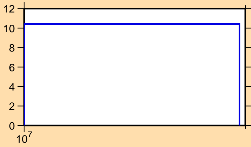
\Delta\sigma/\sigma vs. E for ^{138}\text{Sm}(n,\text{tot.})
