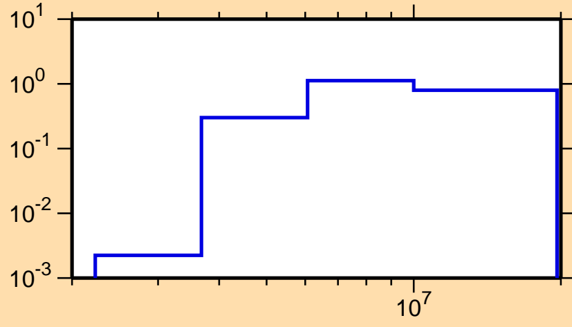
\sigma vs. E for ^{138}\text{Sm}(n,n\text{cont.})
