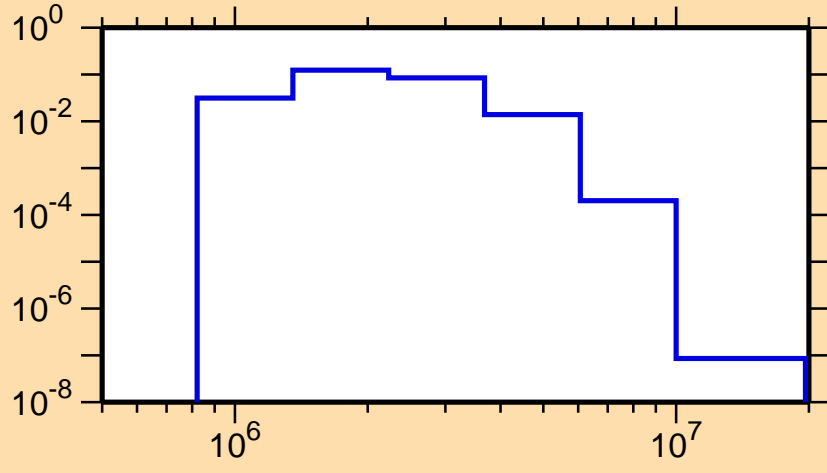
\sigma vs. E for ^{138}\text{Sm}(n,n_4)
