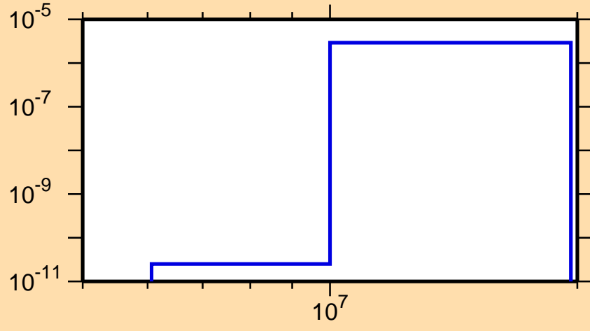
\sigma vs. E for ^{138}\text{Sm}(n,\text{He}3)
