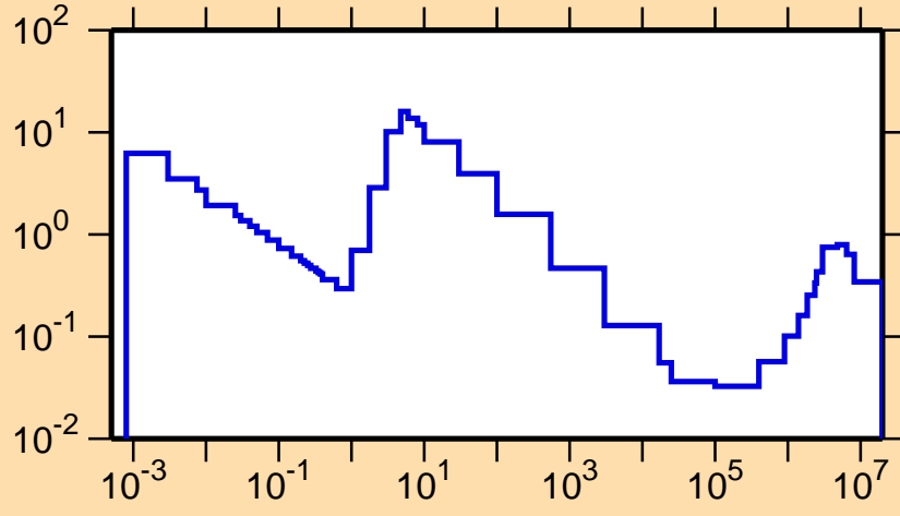
\sigma vs. E for ^{138}\text{Sm}(n,p)
