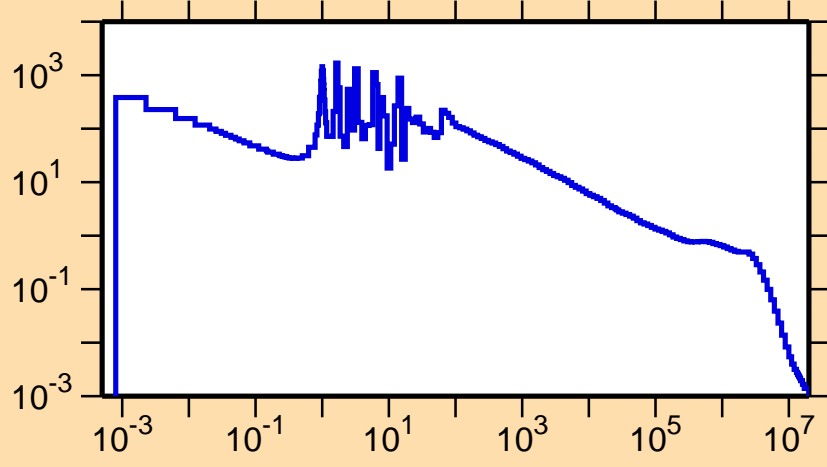
\sigma vs. E for ^{139}\text{Sm}(n,\gamma)
