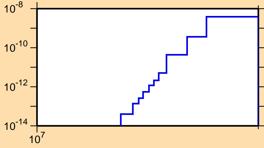
\sigma vs. E for ^{139}\text{Sm}(\text{mt117})
