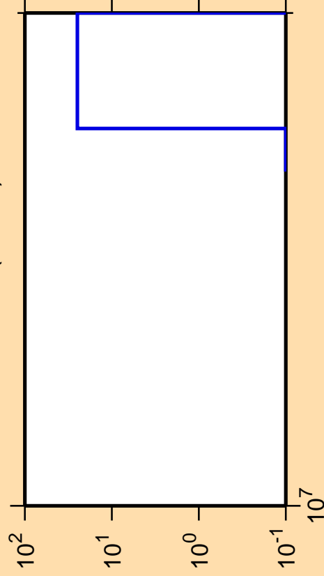
\Delta\sigma/\sigma vs. E for ^{140}\text{Sm} (mt 34)
