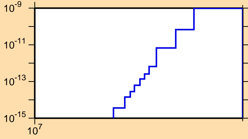
\sigma vs. E for ^{140}\text{Sm}(\text{mt117})
