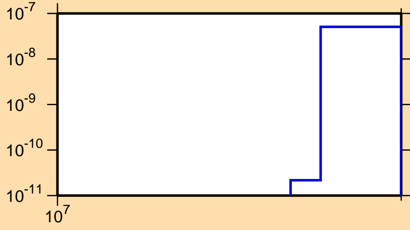
\sigma vs. E for ^{140}\text{Sm}(n,\text{nd})
