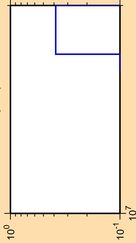
\Delta\sigma/\sigma vs. E for ^{140}\text{Sm}(n,nt)
