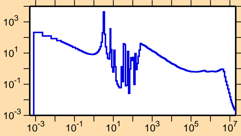
\sigma vs. E for ^{140}\text{Sm}(n,\gamma)
