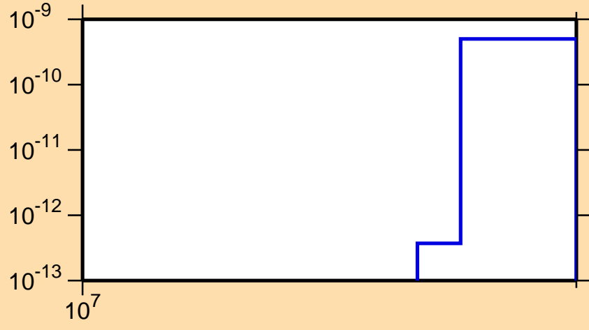
\sigma vs. E for ^{140}\text{Sm}(n,\text{pt})
