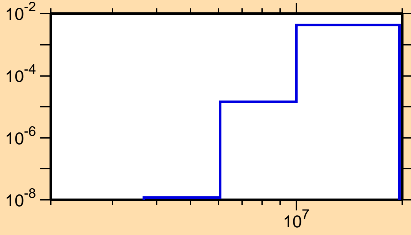
\sigma vs. E for ^{140}\text{Sm}(n,n\alpha)
