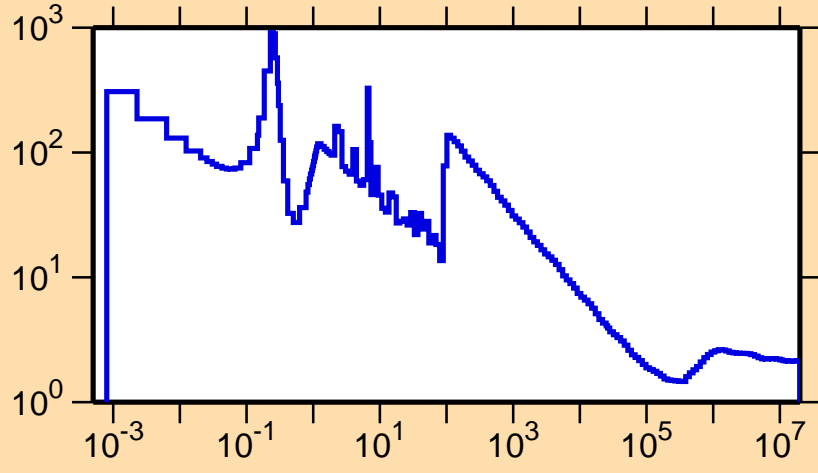
\sigma vs. E for ^{141}\text{Sm}(n,\text{nonel.})
