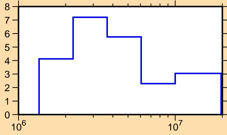
\Delta\sigma/\sigma vs. E for ^{141}\text{Sm}(n, el.)
