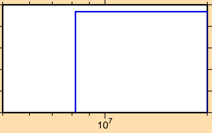
\sigma vs. E for ^{141}\text{Sm}(n,\text{He}3)
