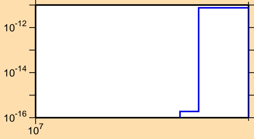
\sigma vs. E for ^{142}\text{Sm}(n,pt)
