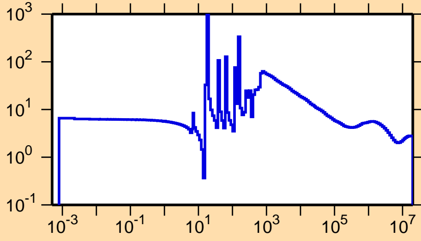
\sigma vs. E for ^{142}\text{Sm}(n,\text{el.})
