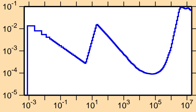
\sigma vs. E for ^{142}\text{Sm}(n,p)
