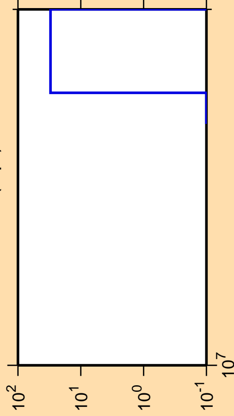
\Delta\sigma/\sigma vs. E for ^{142}\text{Sm}(n,pt)
