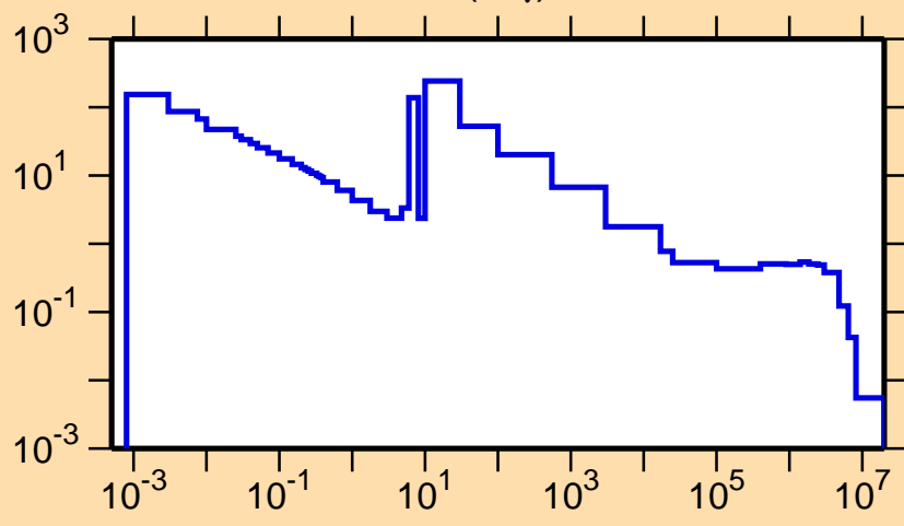
\sigma vs. E for ^{142}\text{Sm}(n,\gamma)
