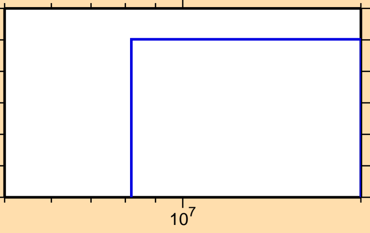
\sigma vs. E for ^{142}\text{Sm} (mt 34)
