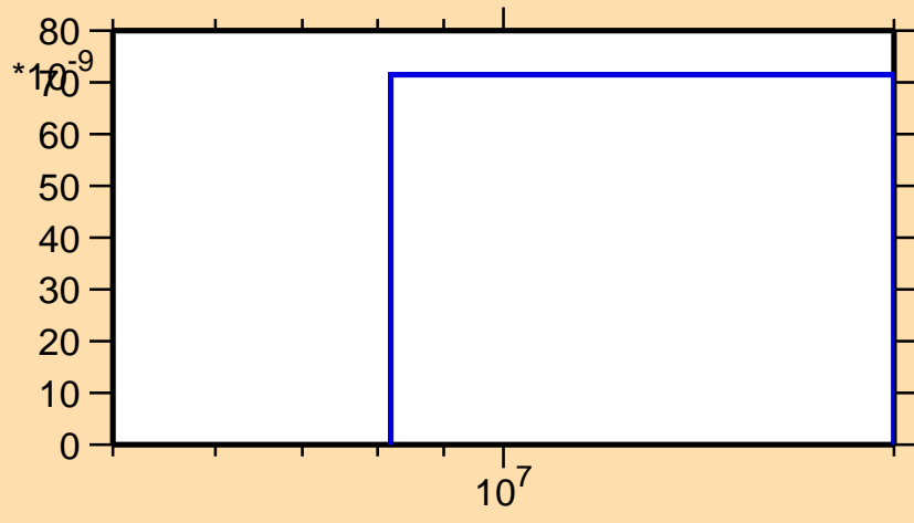
\sigma vs. E for ^{142}\text{Sm}(n,\text{He}3)
