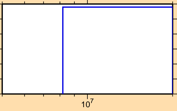
\sigma vs. E for ^{143}\text{Sm}(n,t)
