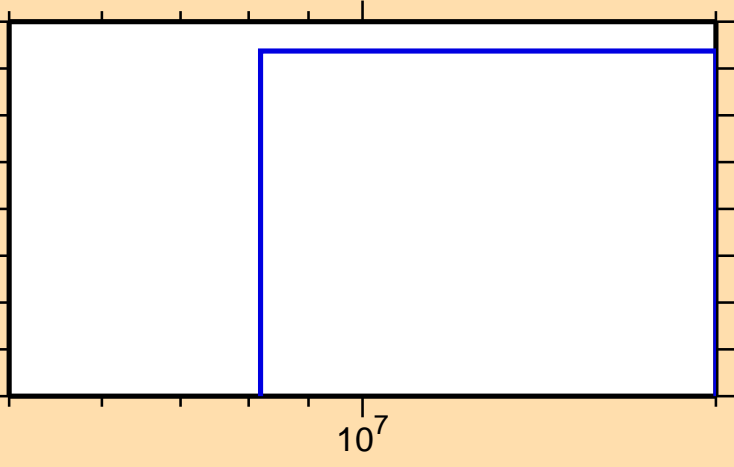
\sigma vs. E for ^{143}\text{Sm}(\text{mt117})
