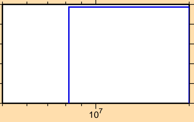
\sigma vs. E for ^{143}\text{Sm}(n,\text{He}3)
