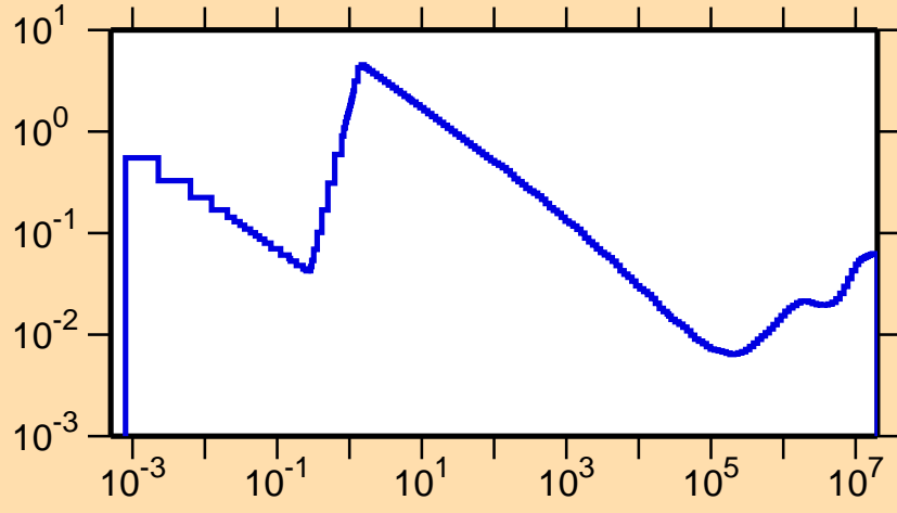
\sigma vs. E for ^{143}\text{Sm}(n,p)
