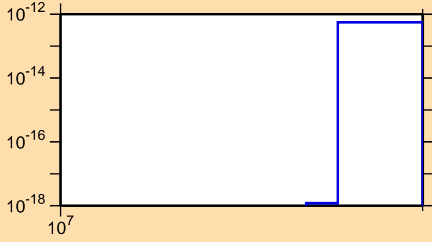
\sigma vs. E for ^{144}\text{Sm}(n,\text{pt})
