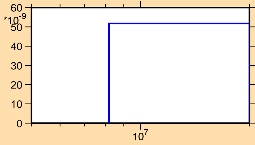
\sigma vs. E for ^{144}\text{Sm}(n,\text{He}3)
