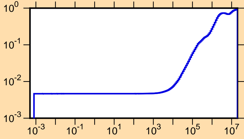
\mu vs. E for ^{145}\text{Sm}(\text{mt251})
