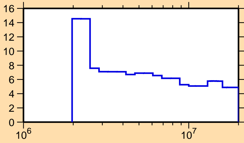
\Delta\sigma/\sigma vs. E for ^{145}\text{Sm}(n,n\text{onel.})
