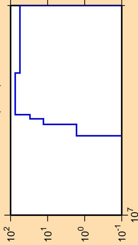
\Delta\sigma/\sigma vs. E for ^{145}\text{Sm}(n,nd)
