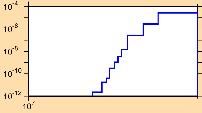
\sigma vs. E for ^{145}\text{Sm}(n,nd)
