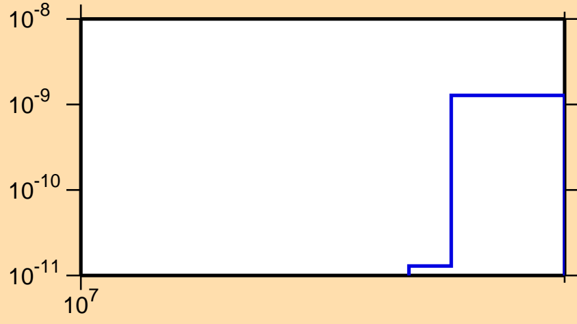
\sigma vs. E for ^{145}\text{Sm}(n,pt)
