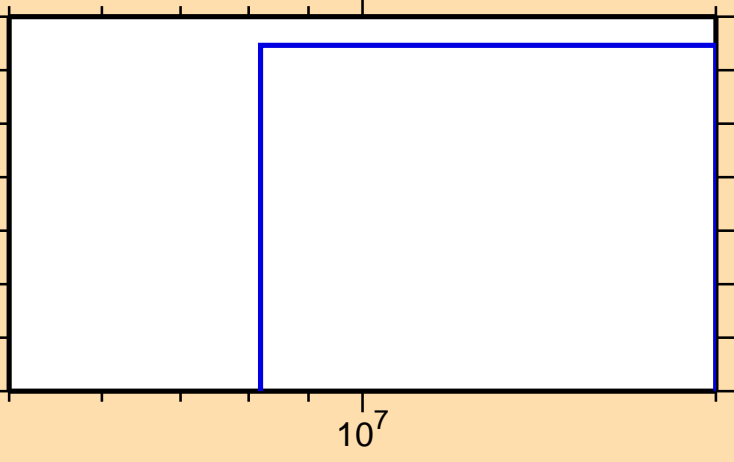
\sigma vs. E for ^{145}\text{Sm}(n,\text{He}3)
