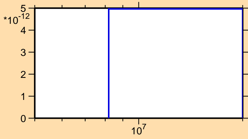
\sigma vs. E for ^{145}\text{Sm}(n,nt)
