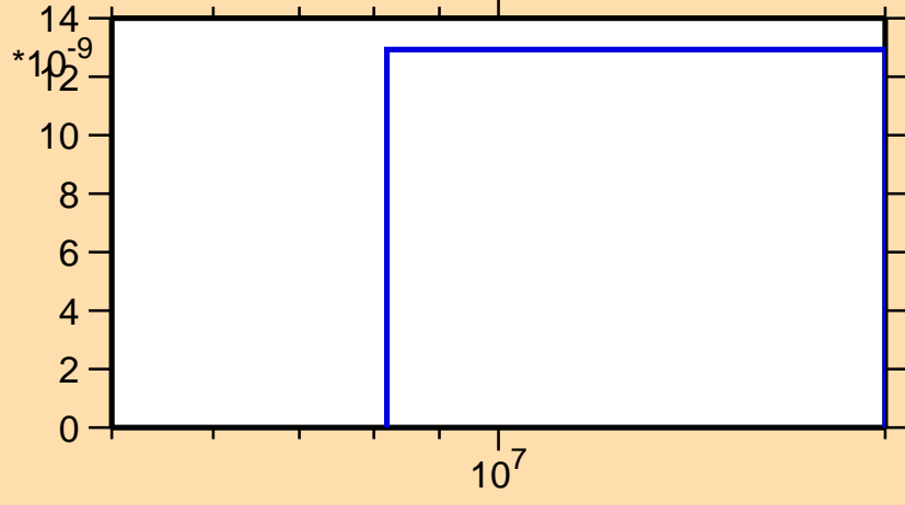
\sigma vs. E for ^{145}\text{Sm}(n,\text{He}3)
