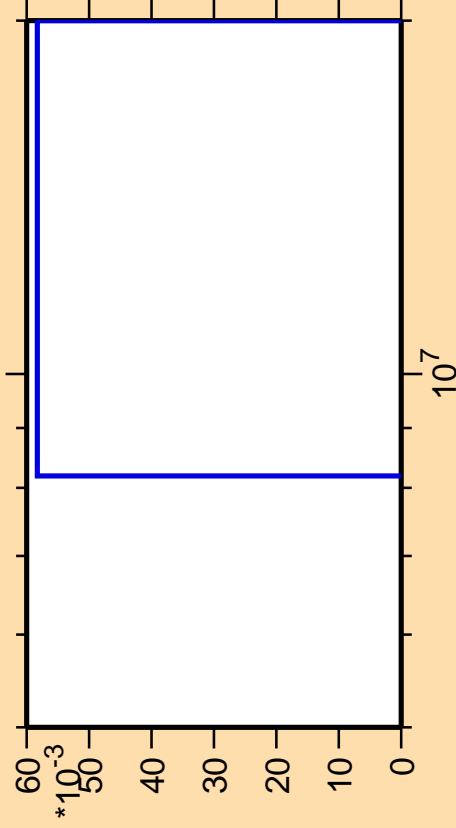
\Delta\sigma/\sigma vs. E for ^{145}\text{Sm}(\text{mt117})
