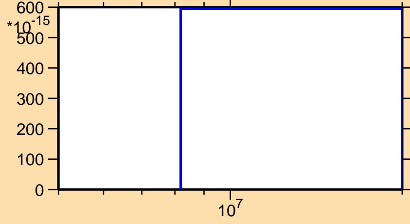
\sigma vs. E for ^{145}\text{Sm}(n,\text{pd})
