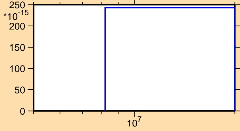
\sigma vs. E for ^{145}\text{Sm} (mt 34)
