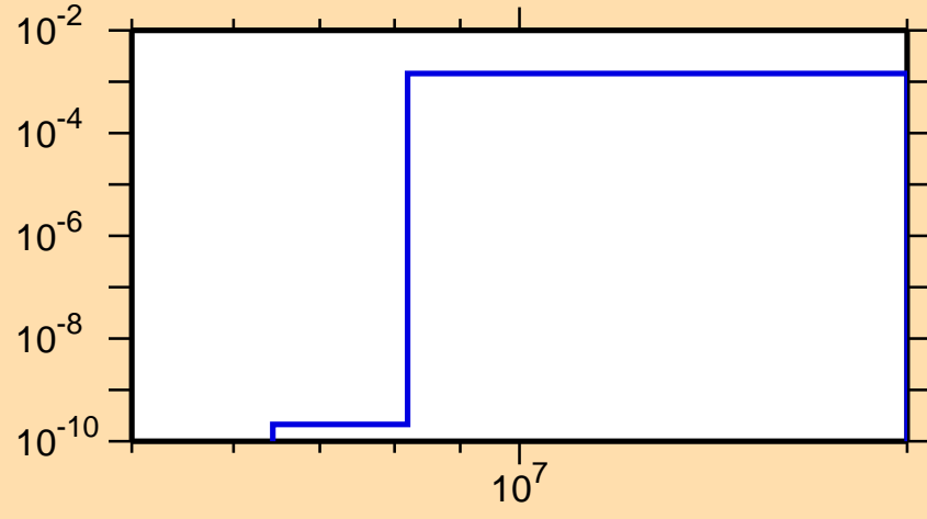
\sigma vs. E for ^{145}\text{Sm}(n,d)
