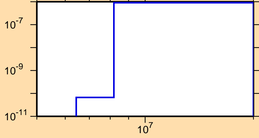
\sigma vs. E for ^{145}\text{Sm}(n,p\alpha)
