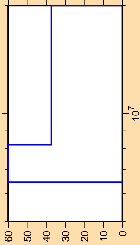
\Delta\sigma/\sigma vs. E for ^{145}\text{Sm}(n,\gamma)
