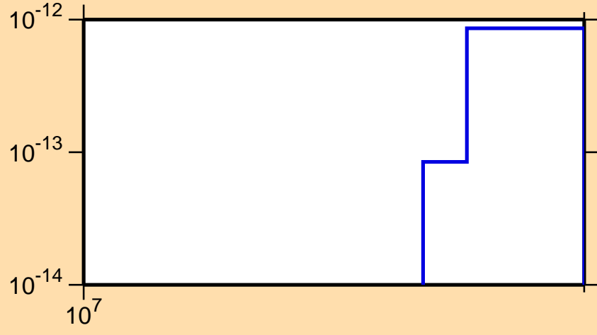
\sigma vs. E for ^{150}\text{Sm}(n,p\alpha)
