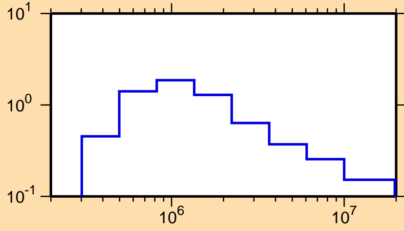
\sigma vs. E for ^{150}\text{Sm}(n,n_1)
