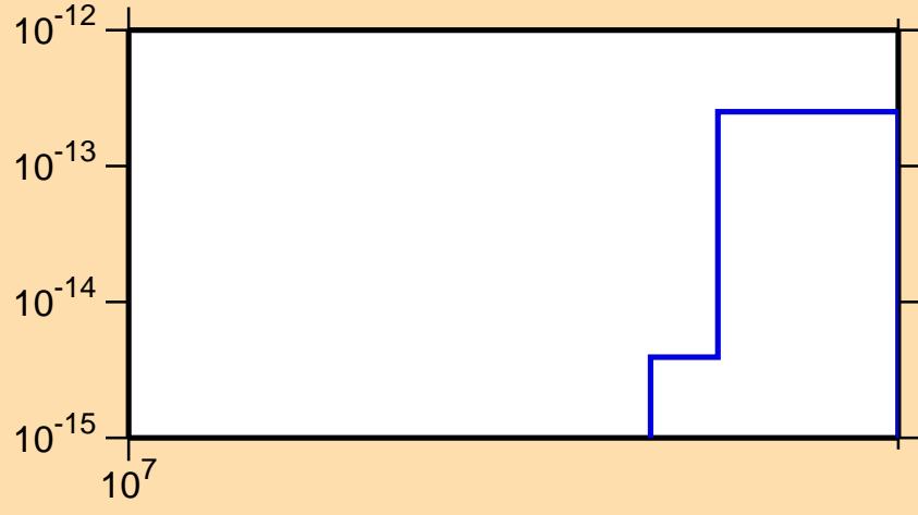
\sigma vs. E for ^{152}\text{Sm}(n,3n\alpha)
