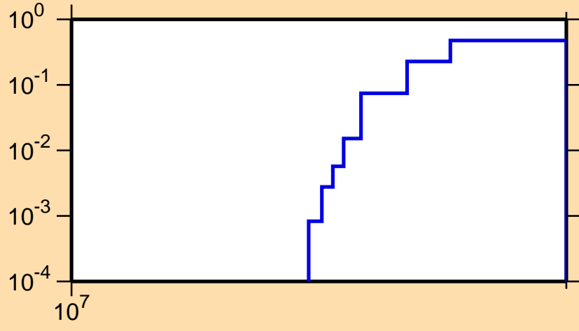
\sigma vs. E for ^{152}\text{Sm}(n,3n)
