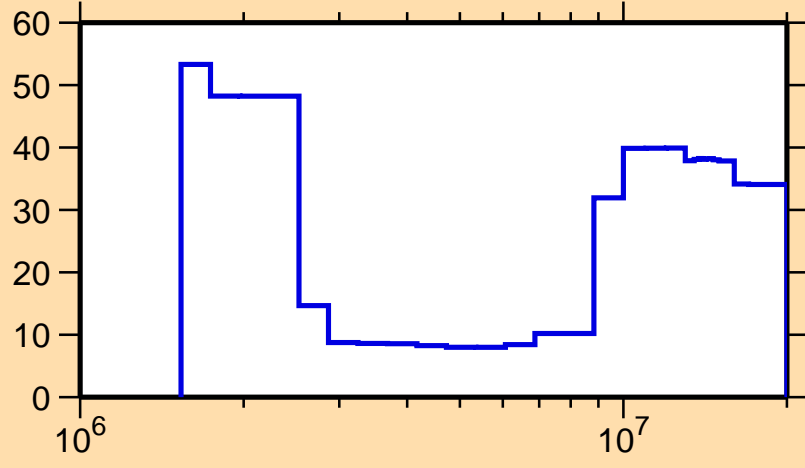
\Delta\sigma/\sigma vs. E for ^{152}\text{Sm}(n,n\text{cont.})
