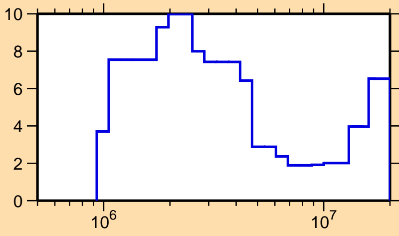
\Delta\sigma/\sigma vs. E for ^{152}\text{Sm}(n,\text{tot.})
