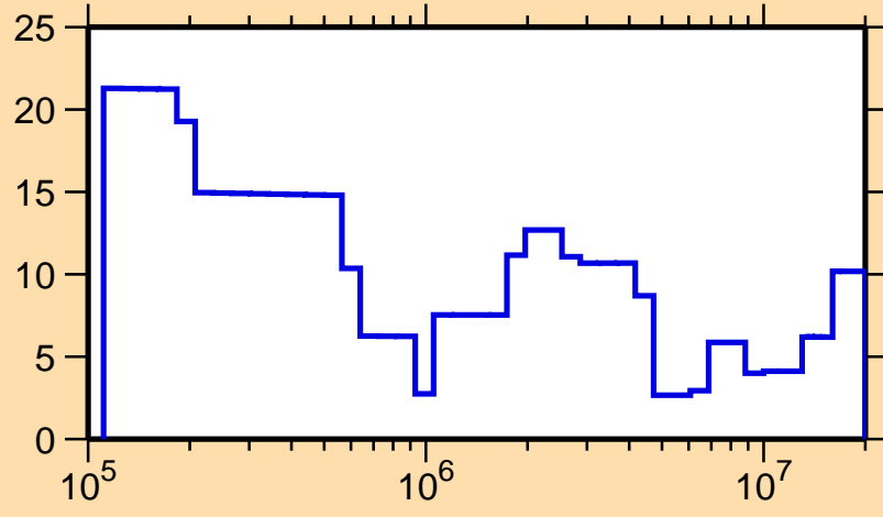
\Delta\sigma/\sigma vs. E for ^{152}\text{Sm}(n,\text{el.})
