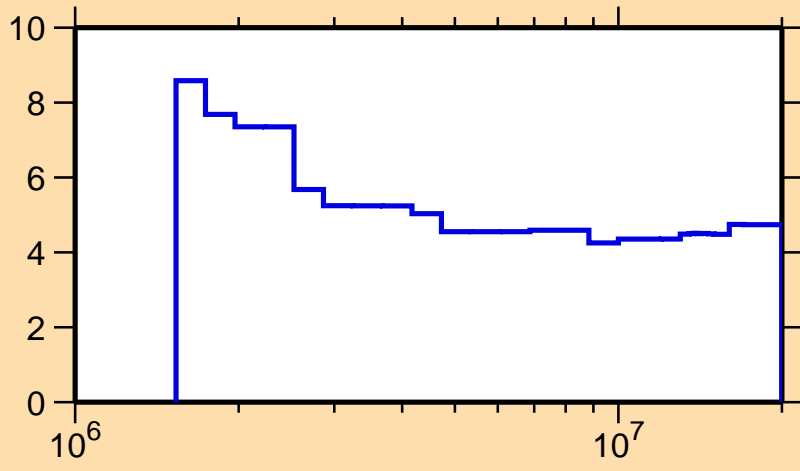
\Delta\sigma/\sigma vs. E for ^{152}\text{Sm}(n,\text{nonel.})
