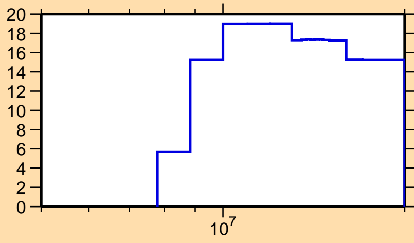
\Delta\sigma/\sigma vs. E for ^{152}\text{Sm}(n,\text{inel.})
