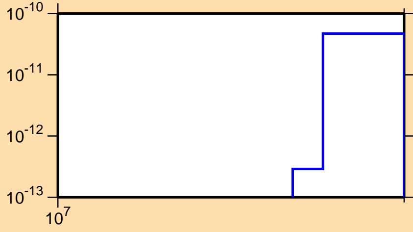
\sigma vs. E for ^{152}\text{Sm}(n,\text{He}3)
