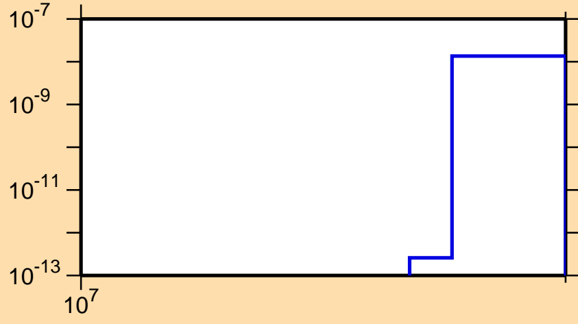
\sigma vs. E for ^{152}\text{Sm}(n,\text{nd})
