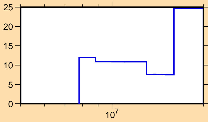
\Delta\sigma/\sigma vs. E for ^{152}\text{Sm}(n,2n)
