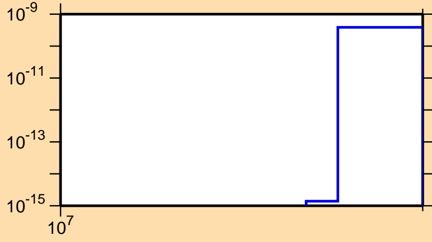
\sigma vs. E for ^{152}\text{Sm}(n,2np)
