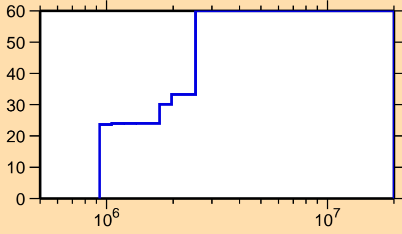
\Delta\sigma/\sigma vs. E for ^{152}\text{Sm}(n,\gamma)
