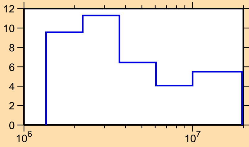
\Delta\sigma/\sigma vs. E for ^{152}\text{Sm}(n, el.)
