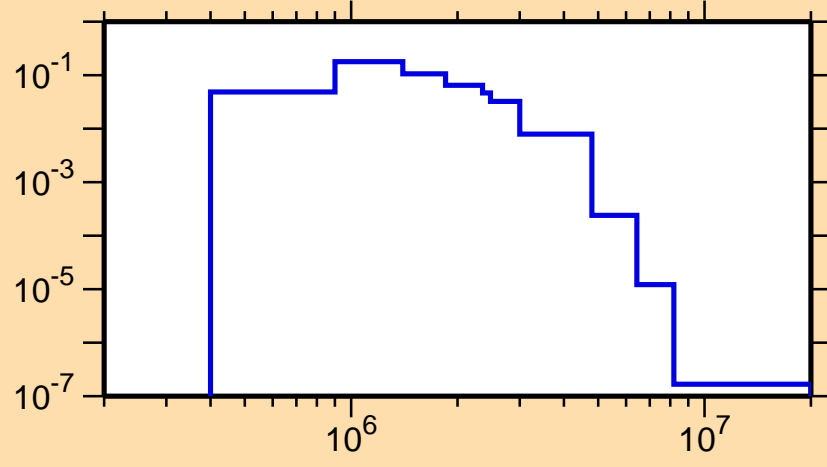
\sigma vs. E for ^{152}\text{Sm}(n,n_3)
