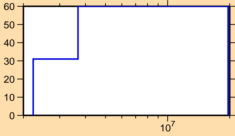
\Delta\sigma/\sigma vs. E for ^{153}\text{Sm}(n,p)
