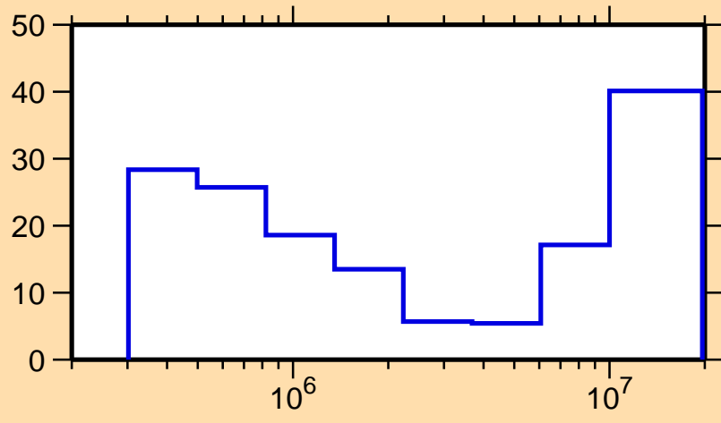
\Delta\sigma/\sigma vs. E for ^{153}\text{Sm}(n,n\text{cont.})
