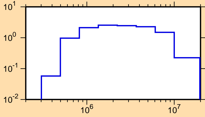
\sigma vs. E for ^{153}\text{Sm}(n,n\text{cont.})
