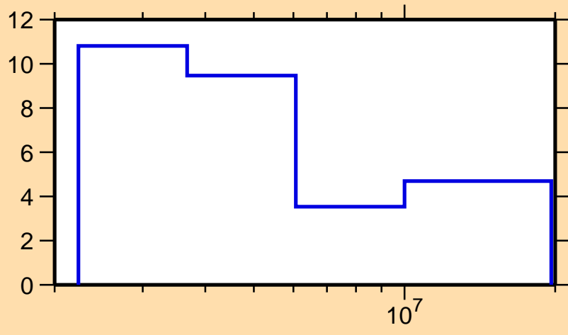
\Delta\sigma/\sigma vs. E for ^{153}\text{Sm}(n,el.)
