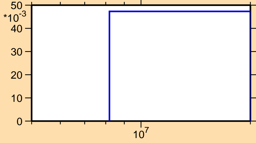
\sigma vs. E for ^{153}\text{Sm}(n,3n)
