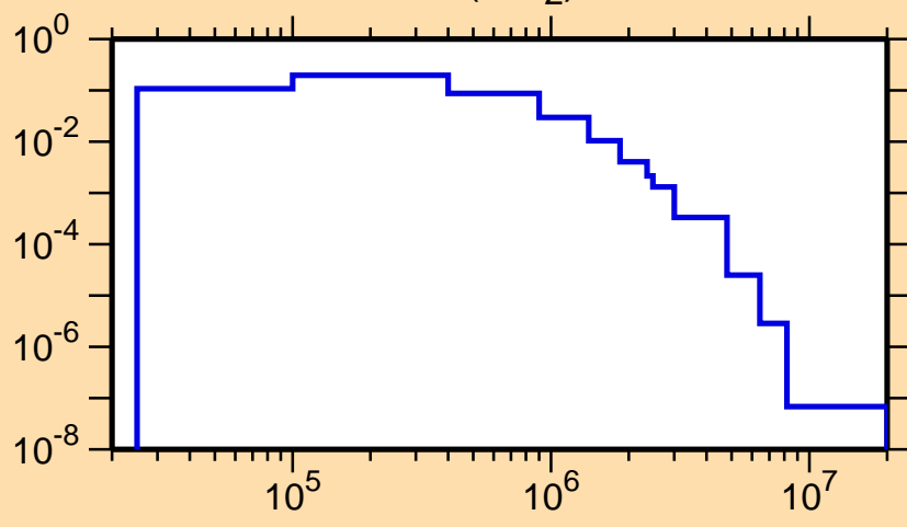
\sigma vs. E for ^{153}\text{Sm}(n,n_2)
