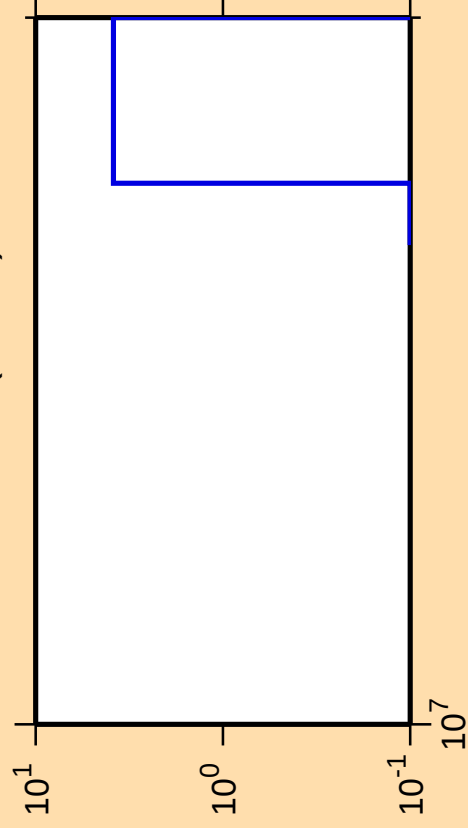
\Delta\sigma/\sigma vs. E for ^{154}\text{Sm}(n,\text{He}3)
