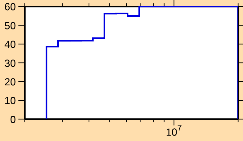
\Delta\sigma/\sigma vs. E for ^{154}\text{Sm}(n,\gamma)
