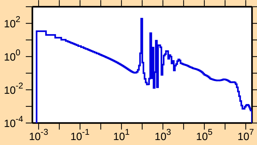
\sigma vs. E for ^{154}\text{Sm}(n,\gamma)
