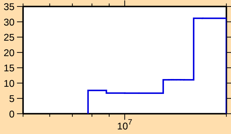
\Delta\sigma/\sigma vs. E for ^{154}\text{Sm}(n,2n)
