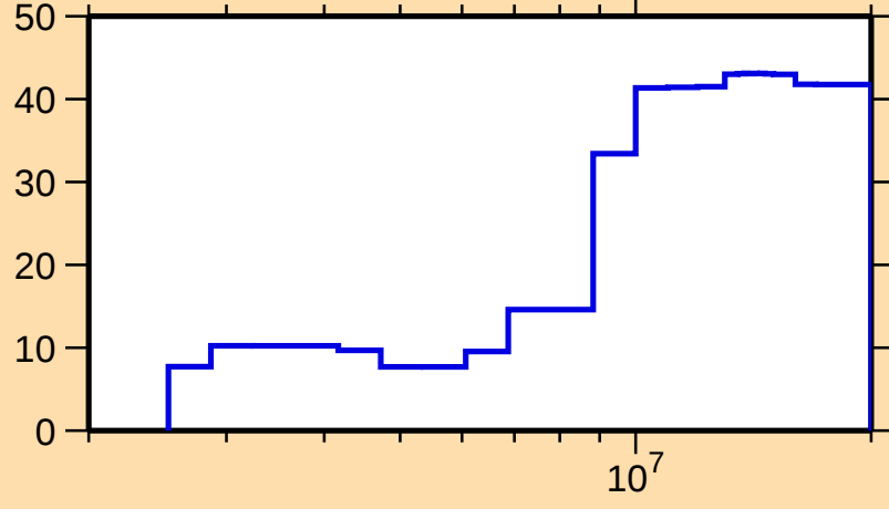
\Delta\sigma/\sigma vs. E for ^{154}\text{Sm}(n,n\text{cont.})
