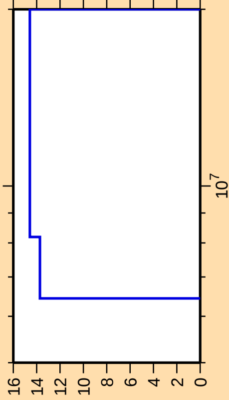
\Delta\sigma/\sigma vs. E for ^{154}\text{Sm}(n,n_1)
