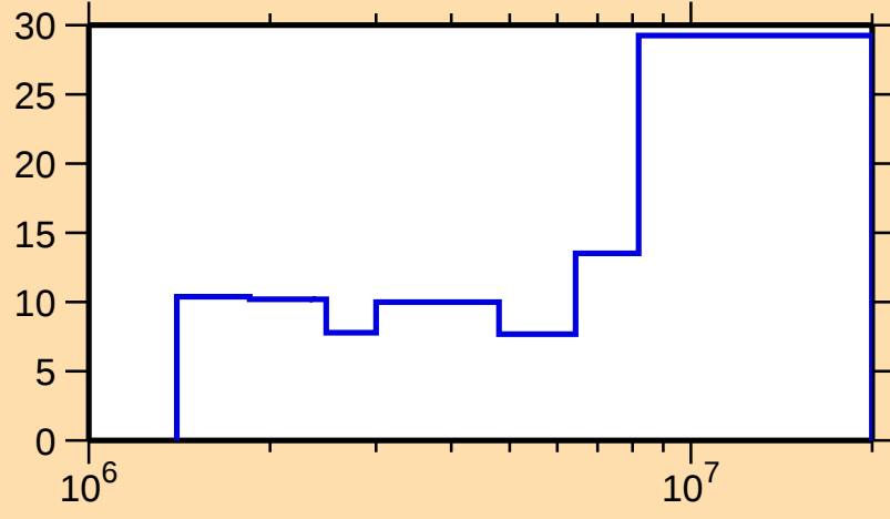
\Delta\sigma/\sigma vs. E for ^{154}\text{Sm}(n,n\text{cont.})
