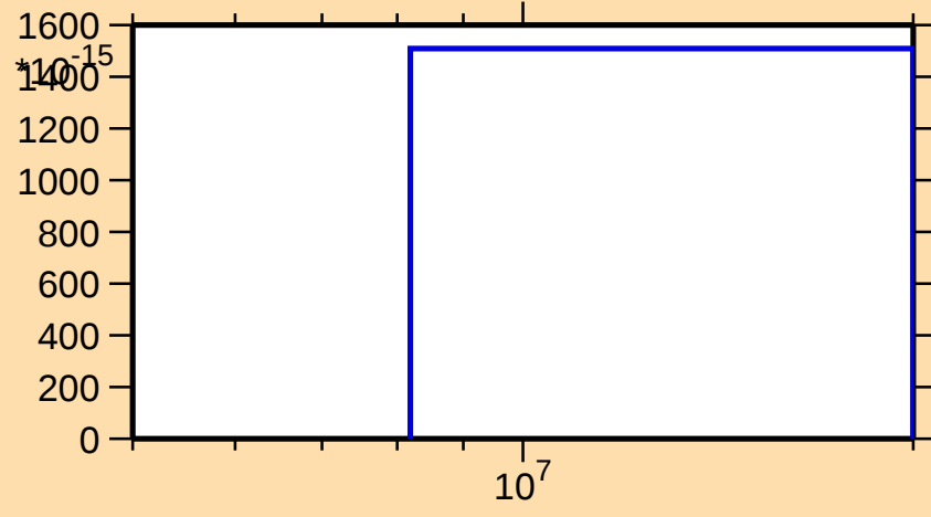
\sigma vs. E for ^{154}\text{Sm}(n,2np)
