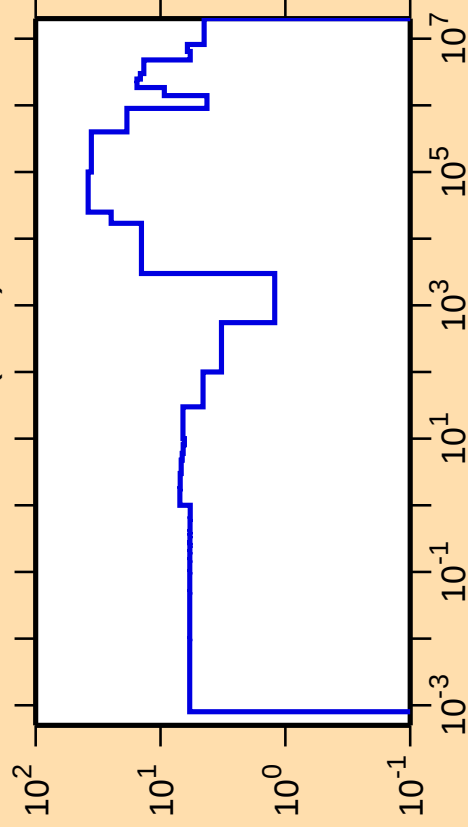
\Delta\sigma/\sigma vs. E for ^{154}\text{Sm}(n,\text{el.})
