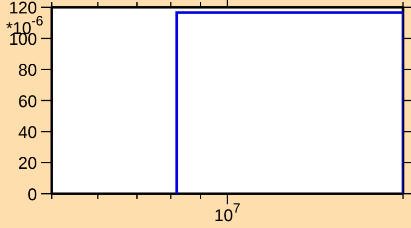
\sigma vs. E for ^{154}\text{Sm}(n,d)
