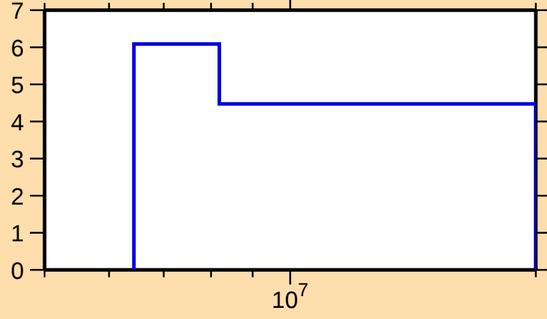
\Delta\sigma/\sigma vs. E for ^{154}\text{Sm}(n,\text{el.})
