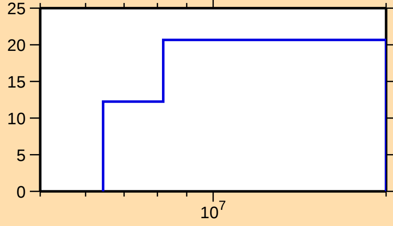
\Delta\sigma/\sigma vs. E for ^{154}\text{Sm}(n,\text{inel.})
