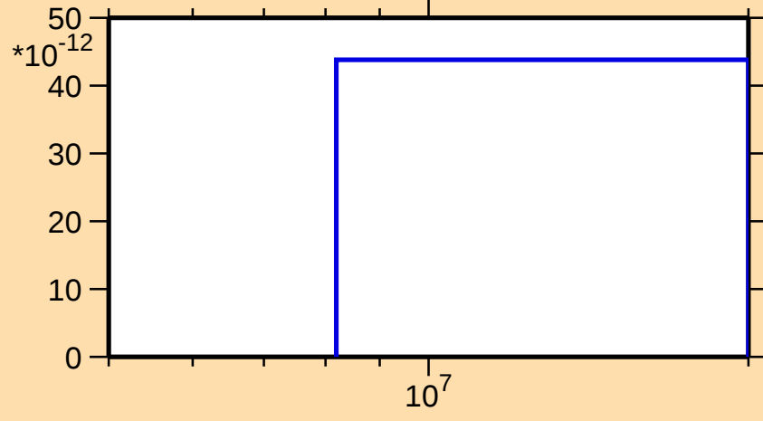
\sigma vs. E for ^{154}\text{Sm}(n,nt)
