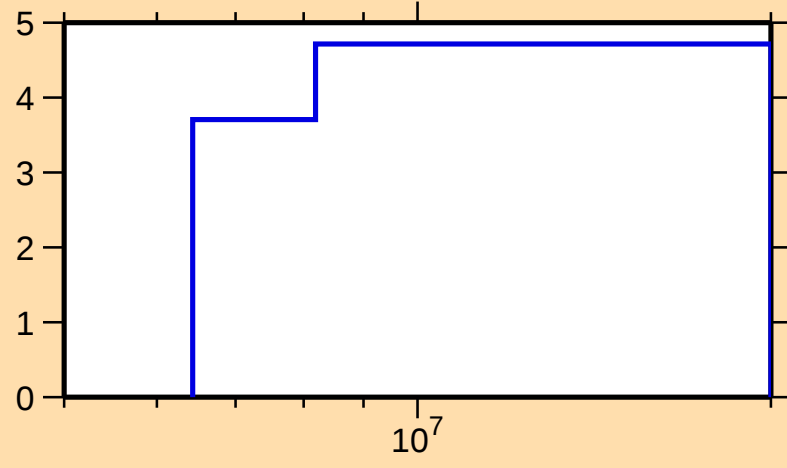
\Delta\sigma/\sigma vs. E for ^{154}\text{Sm}(n,\text{tot.})
