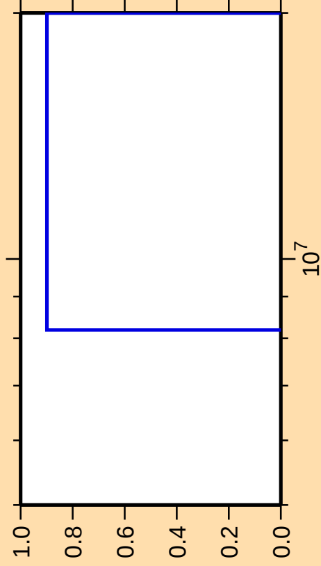
\Delta\sigma/\sigma vs. E for ^{154}\text{Sm}(n,2np)
