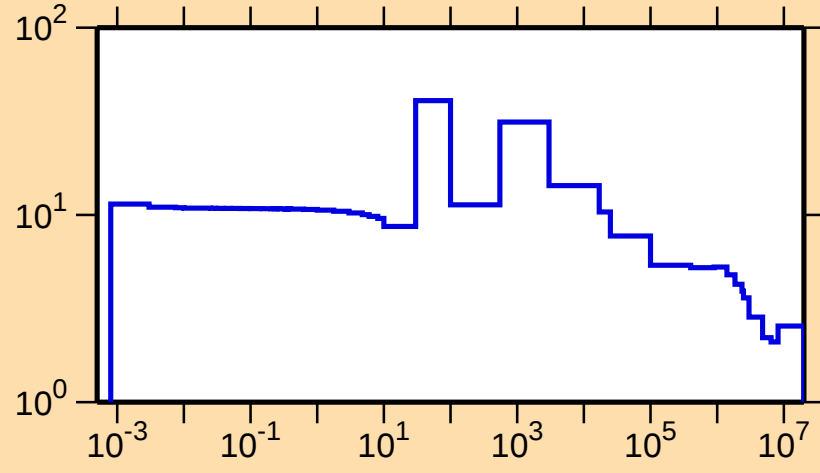
\sigma vs. E for ^{154}\text{Sm}(n,\text{el.})
