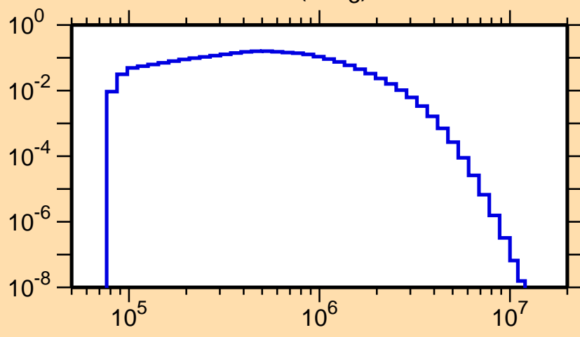
\sigma vs. E for ^{155}\text{Sm}(n,n_3)
