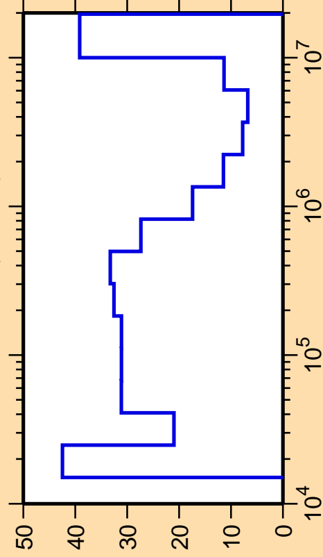
\Delta\sigma/\sigma vs. E for ^{155}\text{Sm}(n,\text{inel.})
