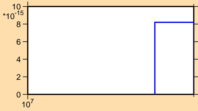
\sigma vs. E for ^{156}\text{Sm}(n,\text{He}3)
