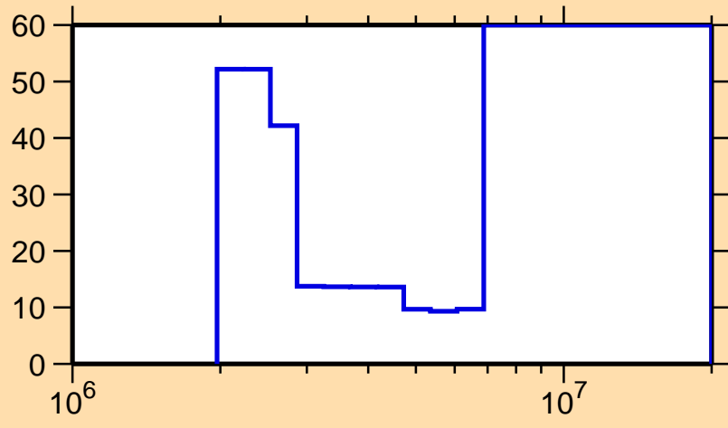
\Delta\sigma/\sigma vs. E for ^{156}\text{Sm}(n,n\text{cont.})
