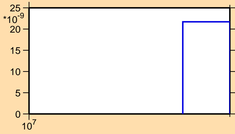
\sigma vs. E for ^{156}\text{Sm}(n,\text{nd})
