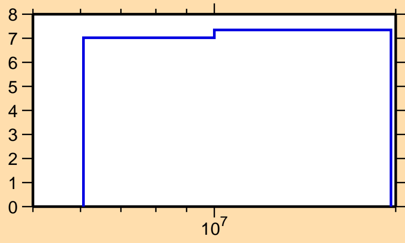
\Delta\sigma/\sigma vs. E for ^{156}\text{Sm}(n,\text{tot.})
