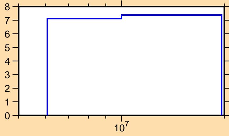
\Delta\sigma/\sigma vs. E for ^{156}\text{Sm}(n,\text{nonel.})
