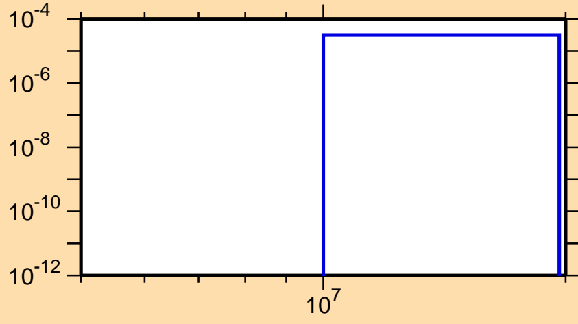
\sigma vs. E for ^{156}\text{Sm}(n,d)
