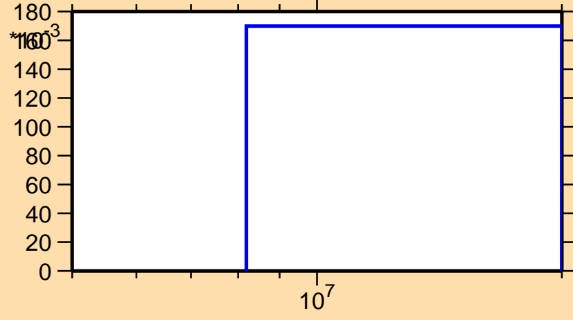
\sigma vs. E for ^{156}\text{Sm}(n,3n)
