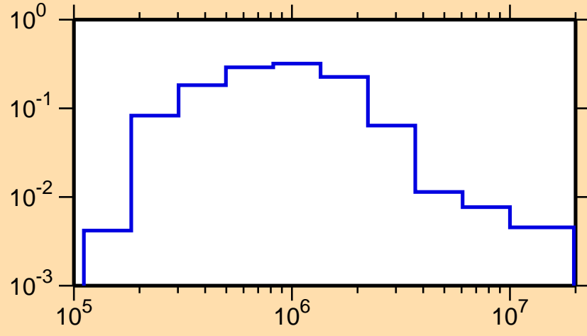
\sigma vs. E for ^{157}\text{Sm}(n,n_3)
