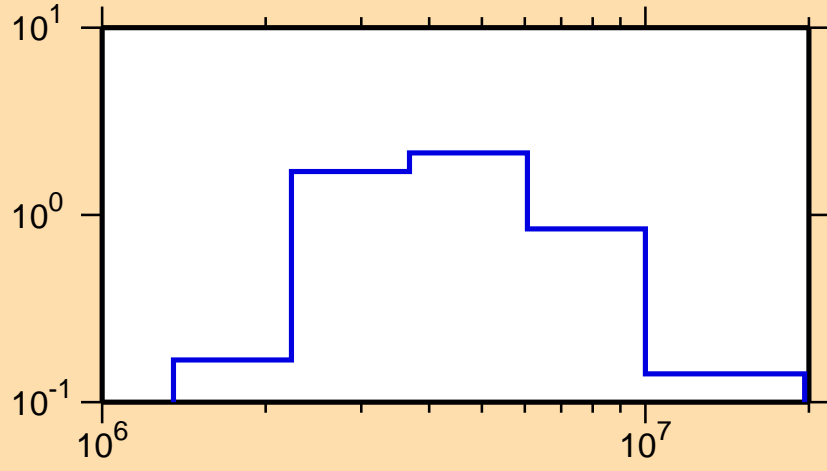
\sigma vs. E for ^{157}\text{Sm}(n,n\text{cont.})
