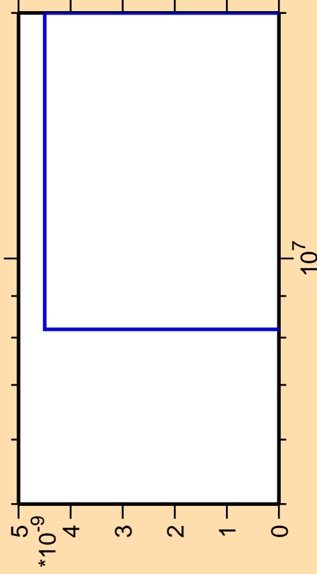
\Delta\sigma/\sigma vs. E for ^{157}\text{Sm} (mt 11)
