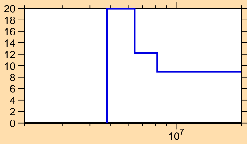
\Delta\sigma/\sigma vs. E for ^{157}\text{Sm}(n,\text{tot.})
