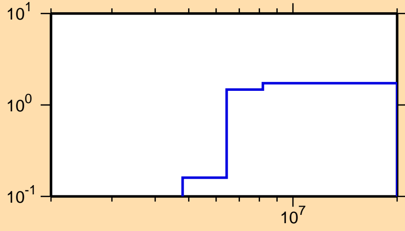
\sigma vs. E for ^{157}\text{Sm}(n,2n)
