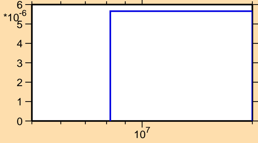
\sigma vs. E for ^{157}\text{Sm}(n,\alpha)
