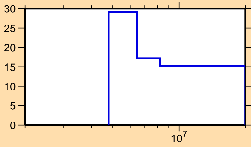
\Delta\sigma/\sigma vs. E for ^{157}\text{Sm}(n,2n)
