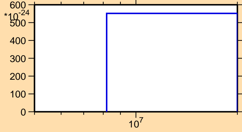
\sigma vs. E for ^{157}\text{Sm} (mt 11)
