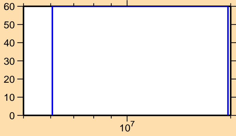
\Delta\sigma/\sigma vs. E for ^{158}\text{Sm}(n,p)
