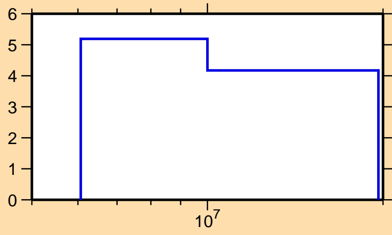
\Delta\sigma/\sigma vs. E for ^{158}\text{Sm}(n,\text{nonel.})
