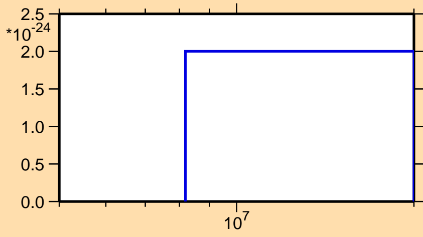
\sigma vs. E for ^{158}\text{Sm}(\text{mt } 11)
