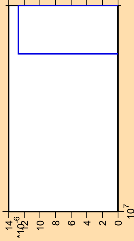
\Delta\sigma/\sigma vs. E for ^{159}\text{Sm} (mt 11)
