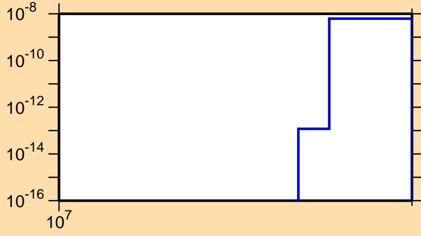
\sigma vs. E for ^{159}\text{Sm}(n,2np)
