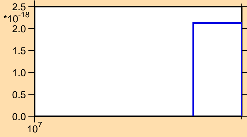
\sigma vs. E for ^{159}\text{Sm} (mt 11)
