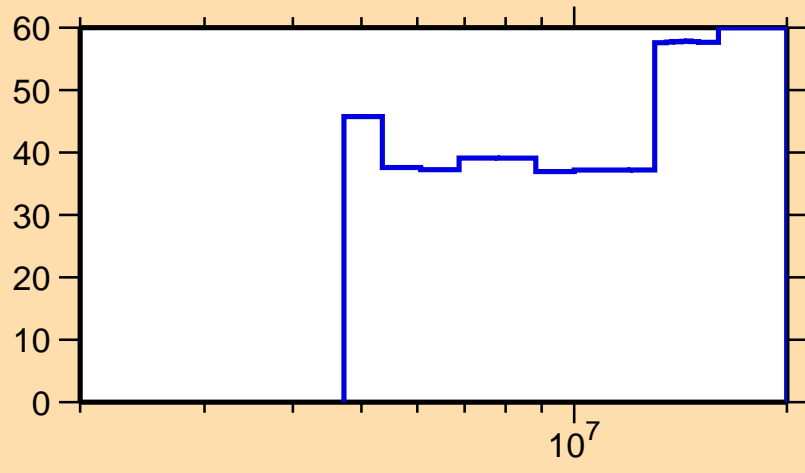
\Delta\sigma/\sigma vs. E for ^{159}\text{Sm}(n,2n)
