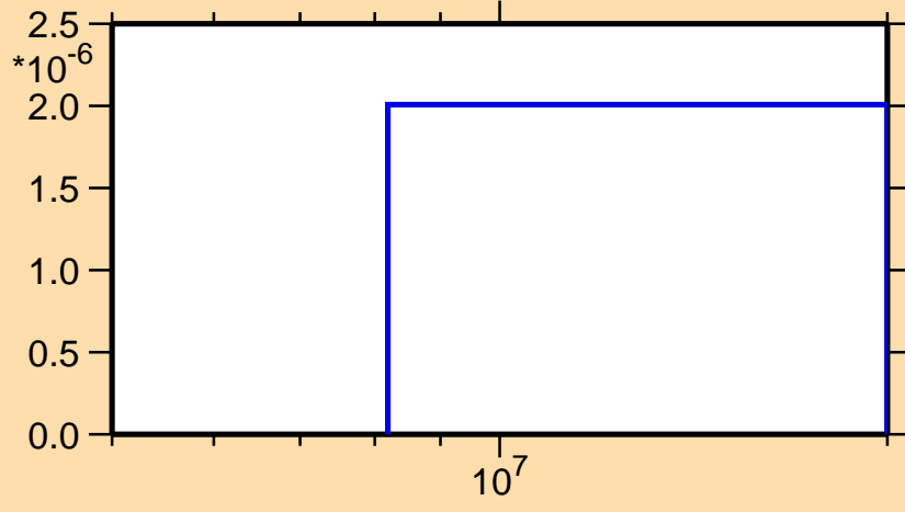
\sigma vs. E for ^{159}\text{Sm}(n,\alpha)
