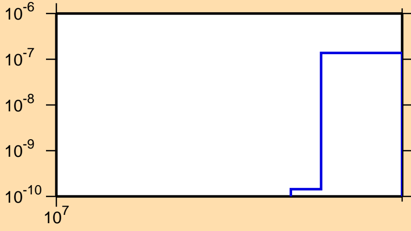
\sigma vs. E for ^{160}\text{Sm}(n,nt)
