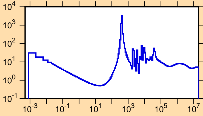
\sigma vs. E for ^{160}\text{Sm}(n,\text{tot.})
