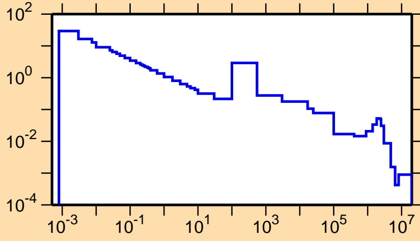
\sigma vs. E for ^{160}\text{Sm}(n,\gamma)
