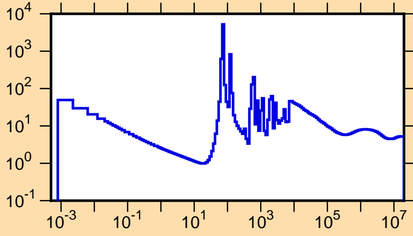
\sigma vs. E for ^{161}\text{Sm}(n,\text{tot.})
