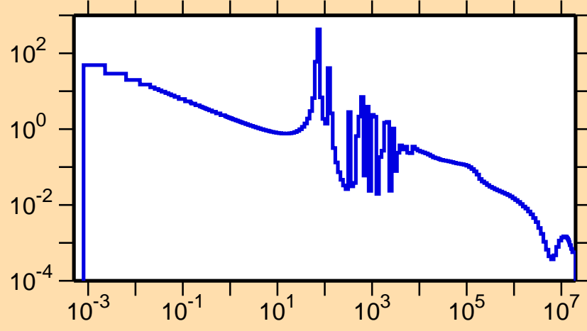
\sigma vs. E for ^{161}\text{Sm}(n,\gamma)
