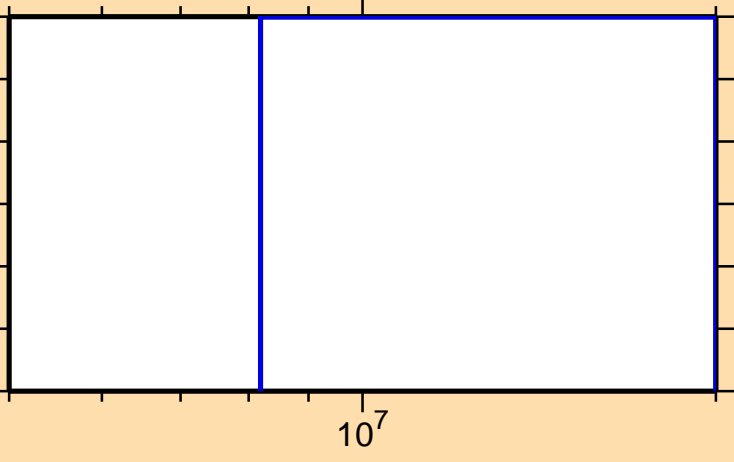
\sigma vs. E for ^{161}\text{Sm}(n,d)
