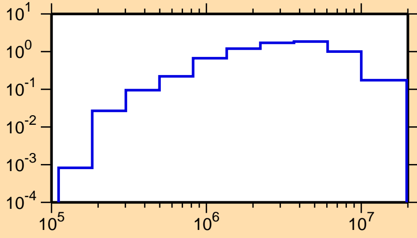
\sigma vs. E for ^{162}\text{Sm}(n,n\text{cont.})
