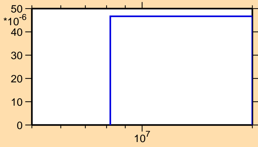
\sigma vs. E for ^{162}\text{Sm}(n,p)
