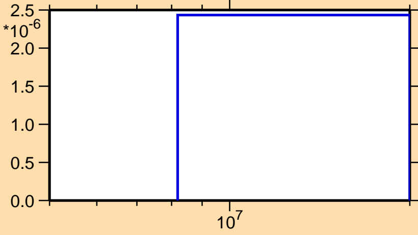
\sigma vs. E for ^{162}\text{Sm}(n,t)
