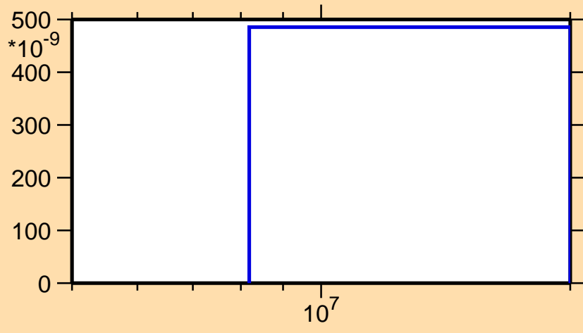
\sigma vs. E for ^{162}\text{Sm}(n,np)
