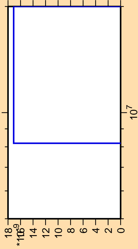
\Delta\sigma/\sigma vs. E for ^{162}\text{Sm}(\text{mt } 11)
