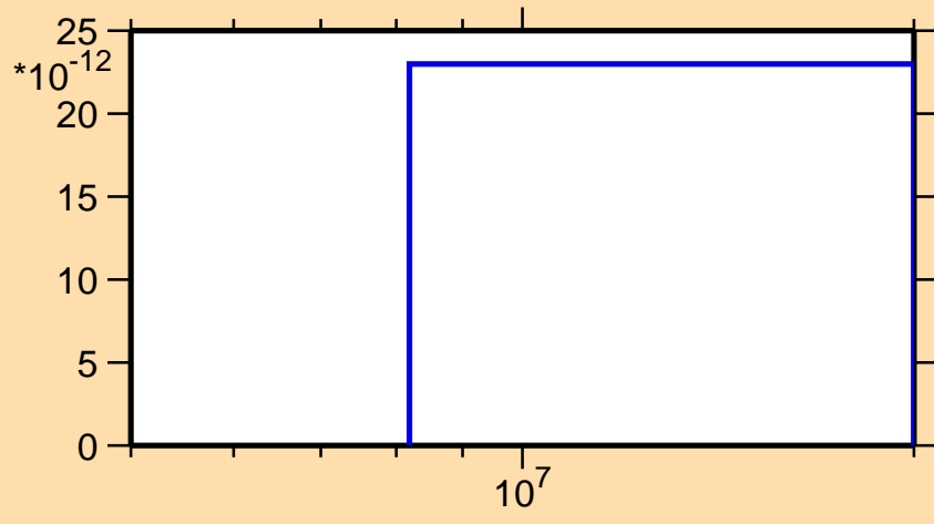
\sigma vs. E for ^{162}\text{Sm}(n,\text{nd})
