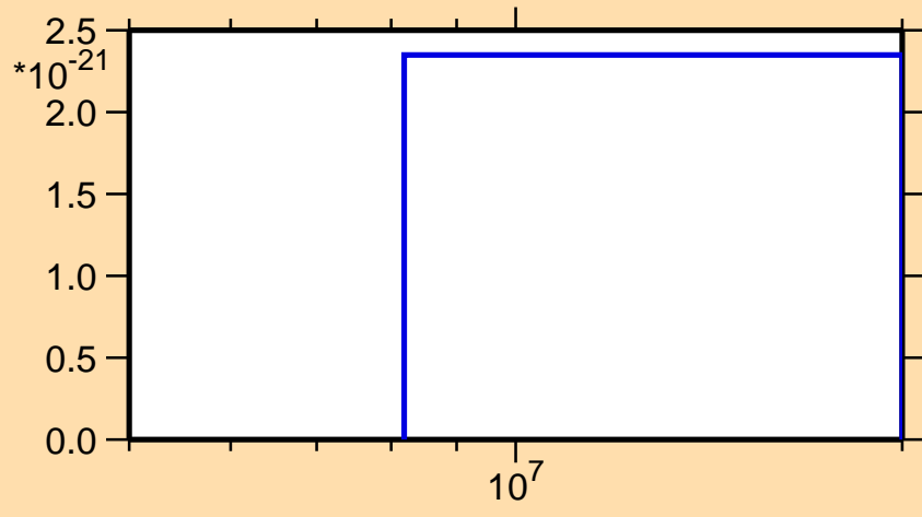
\sigma vs. E for ^{162}\text{Sm}(\text{mt } 11)
