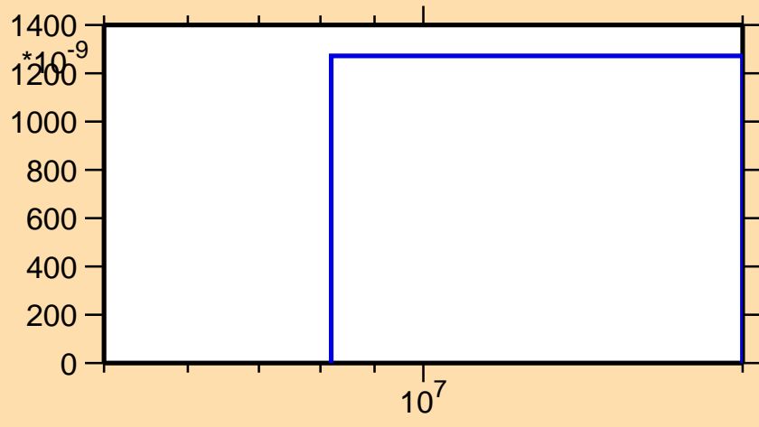
\sigma vs. E for ^{162}\text{Sm}(n,d)
