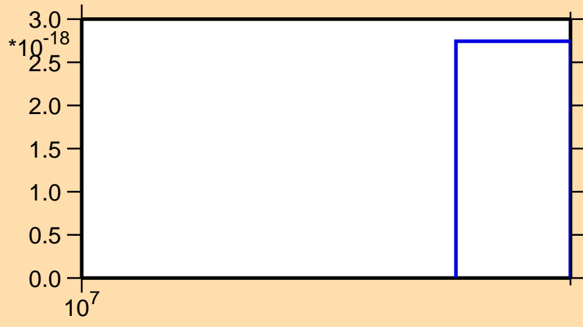
\sigma vs. E for ^{163}\text{Sm} (mt 11)
