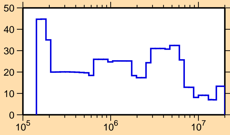
\Delta\sigma/\sigma vs. E for ^{163}\text{Sm}(n,\text{el.})
