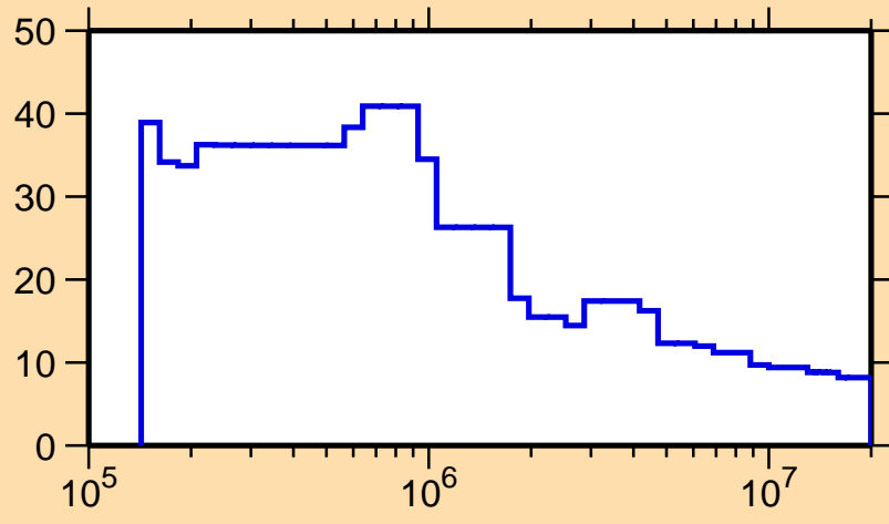
\Delta\sigma/\sigma vs. E for ^{163}\text{Sm}(n,\text{nonel.})
