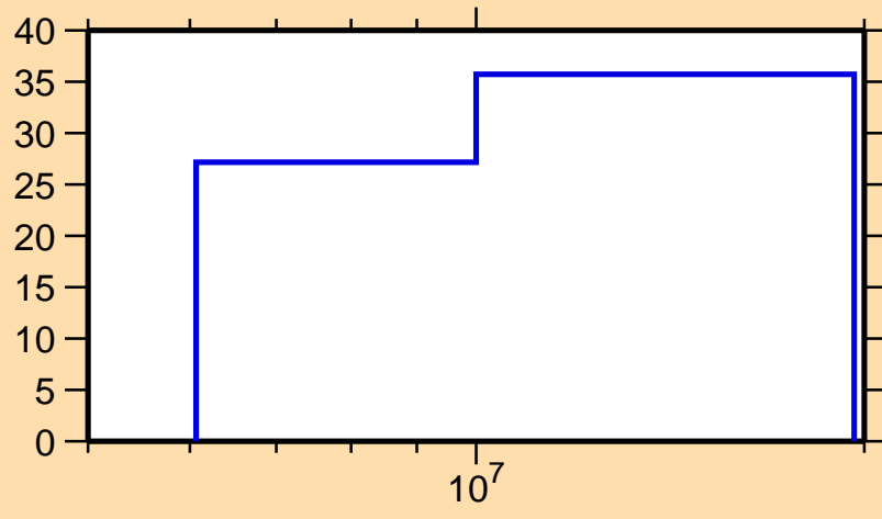
\Delta\sigma/\sigma vs. E for ^{163}\text{Sm}(n,2n)
