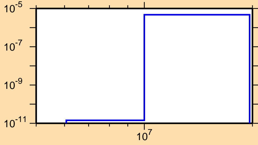
\sigma vs. E for ^{163}\text{Sm}(n,\alpha)
