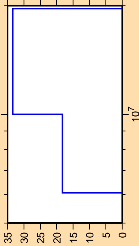
\Delta\sigma/\sigma vs. E for ^{163}\text{Sm}(n,p)
