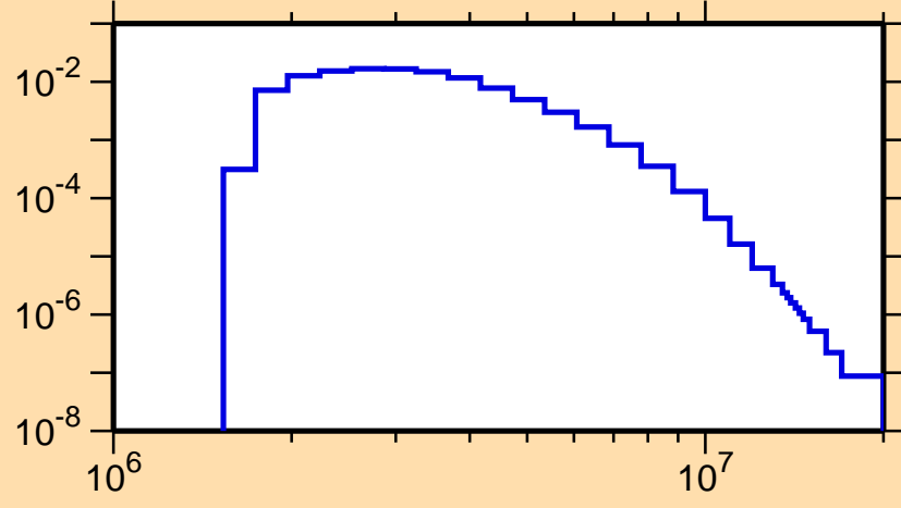
\sigma vs. E for ^{101}\text{Sn}(n,n_4)
