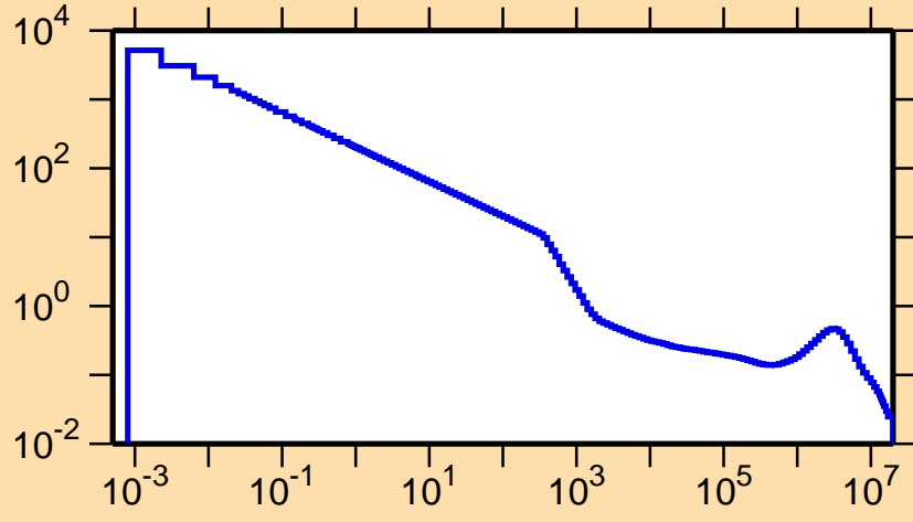
\sigma vs. E for ^{101}\text{Sn}(n,\alpha)
