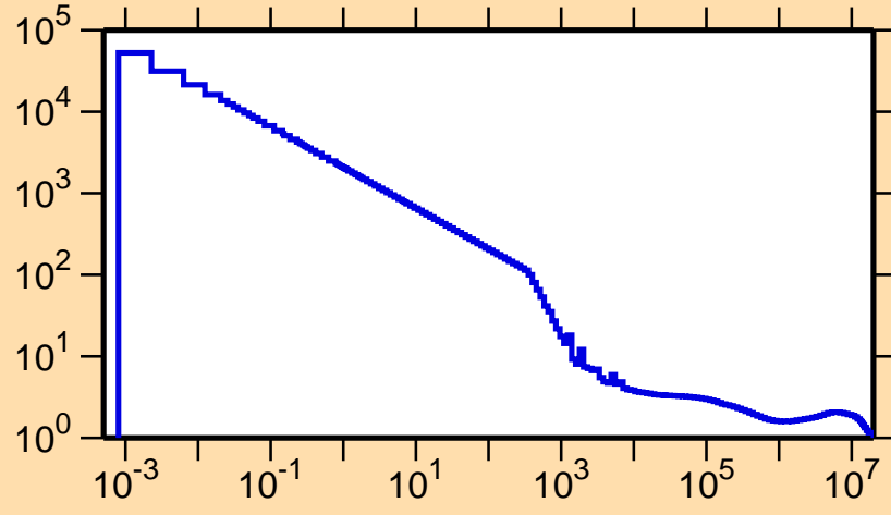
\sigma vs. E for ^{101}\text{Sn}(n,\text{nonel.})
