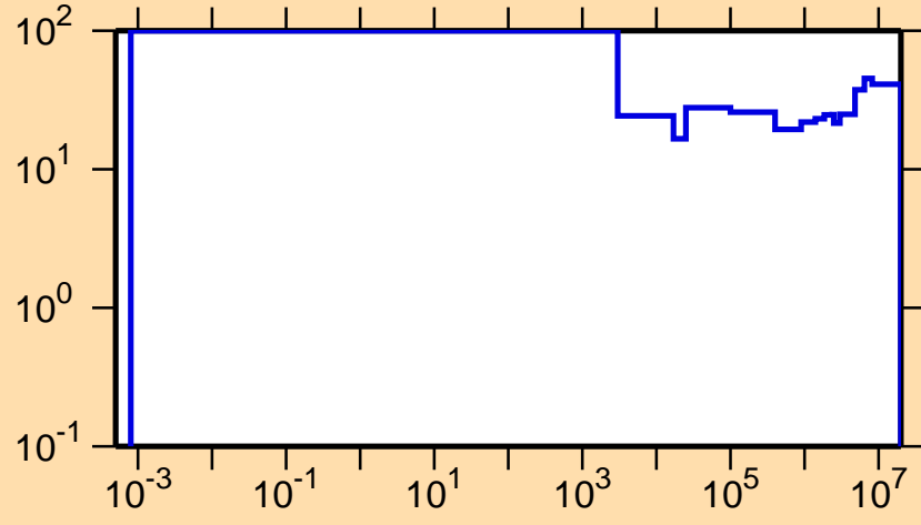
\Delta\sigma/\sigma vs. E for ^{101}\text{Sn}(n,p)
