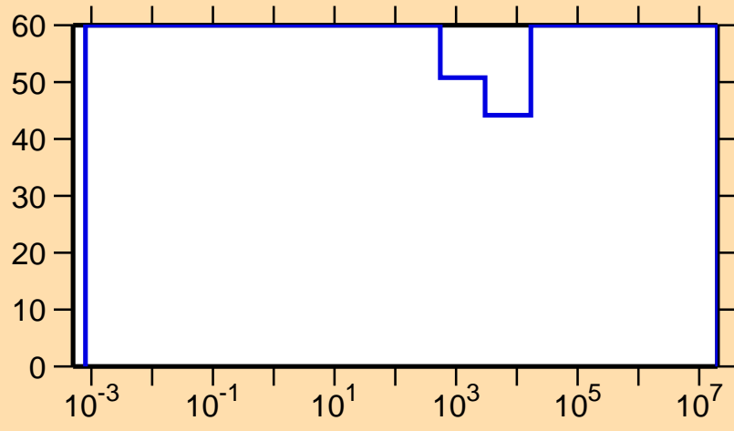
\Delta\sigma/\sigma vs. E for ^{101}\text{Sn}(n,\gamma)
