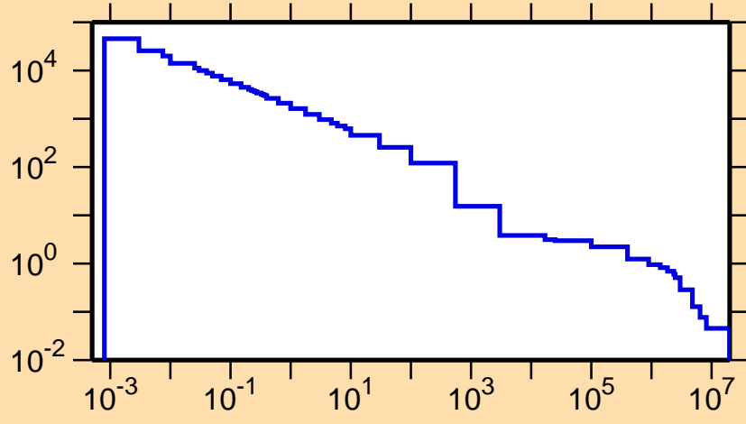
\sigma vs. E for ^{101}\text{Sn}(n,p)
