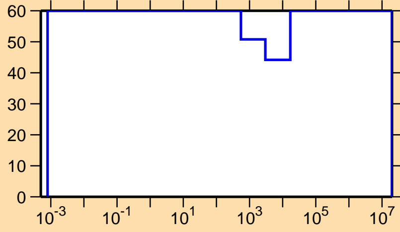
\Delta\sigma/\sigma vs. E for ^{101}\text{Sn}(n,\gamma)
