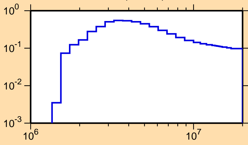
\sigma vs. E for ^{102}\text{Sn}(n,\text{inel.})
