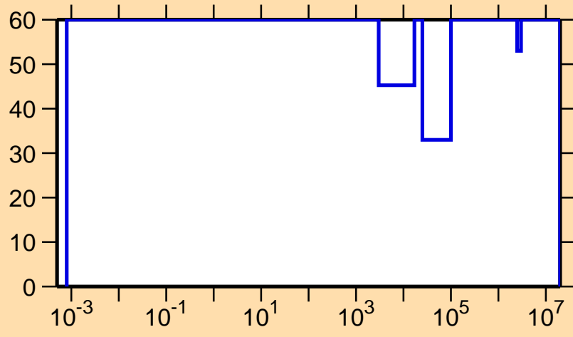
\Delta\sigma/\sigma vs. E for ^{102}\text{Sn}(n,\gamma)
