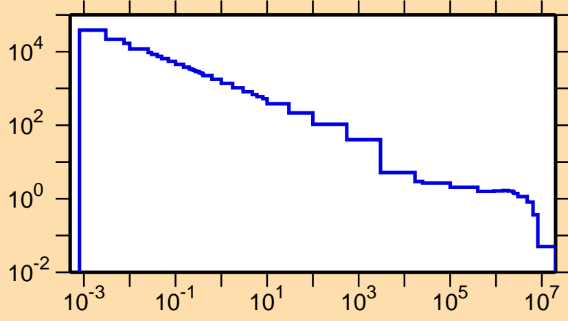
\sigma vs. E for ^{102}\text{Sn}(n,p)
