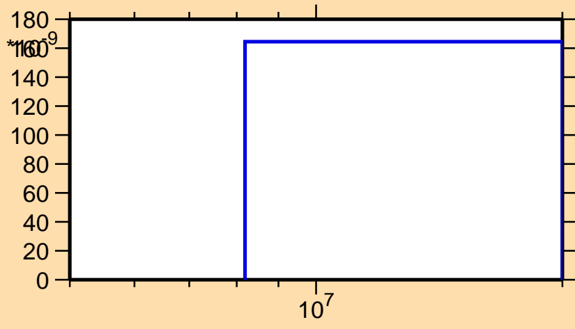
\sigma vs. E for ^{102}\text{Sn}(\text{mt } 45)
