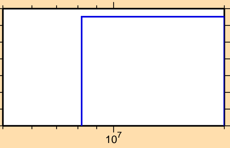
\sigma vs. E for ^{102}\text{Sn}(n,2np)
