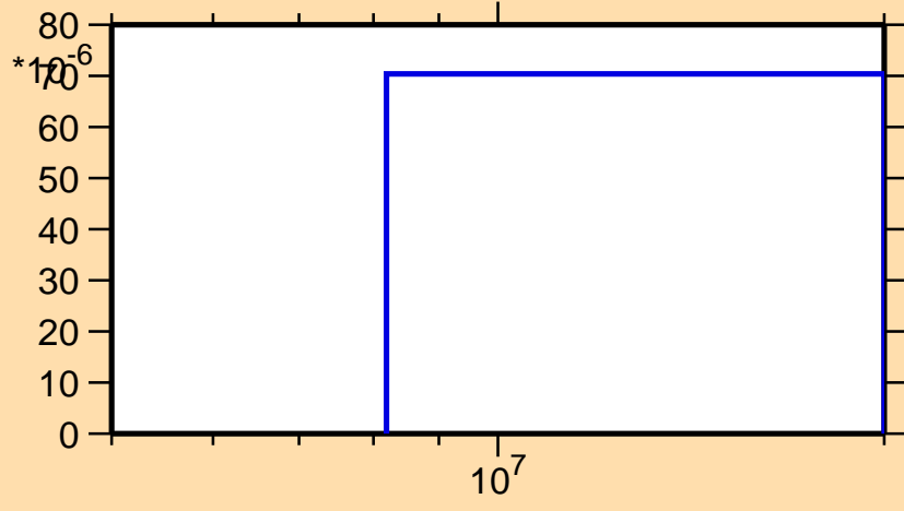
\sigma vs. E for ^{102}\text{Sn}(n,t)
