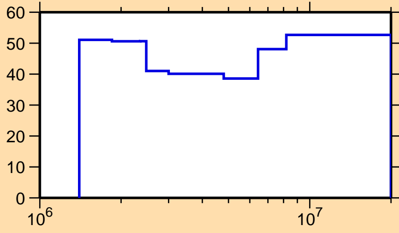
\Delta\sigma/\sigma vs. E for ^{102}\text{Sn}(n,\text{inel.})
